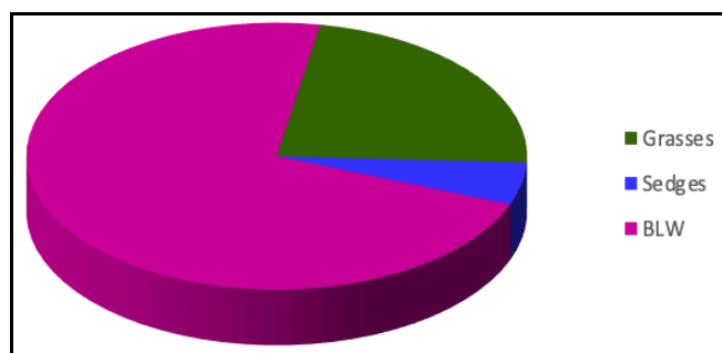
Fig 2: Percentage (%) of groups based on morphological characteristics
